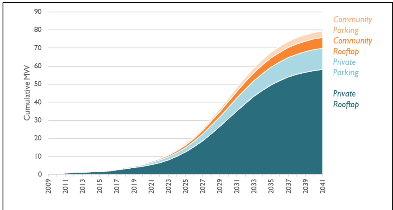
Figure 39. Ward 1 High projection solar potential by installation type
