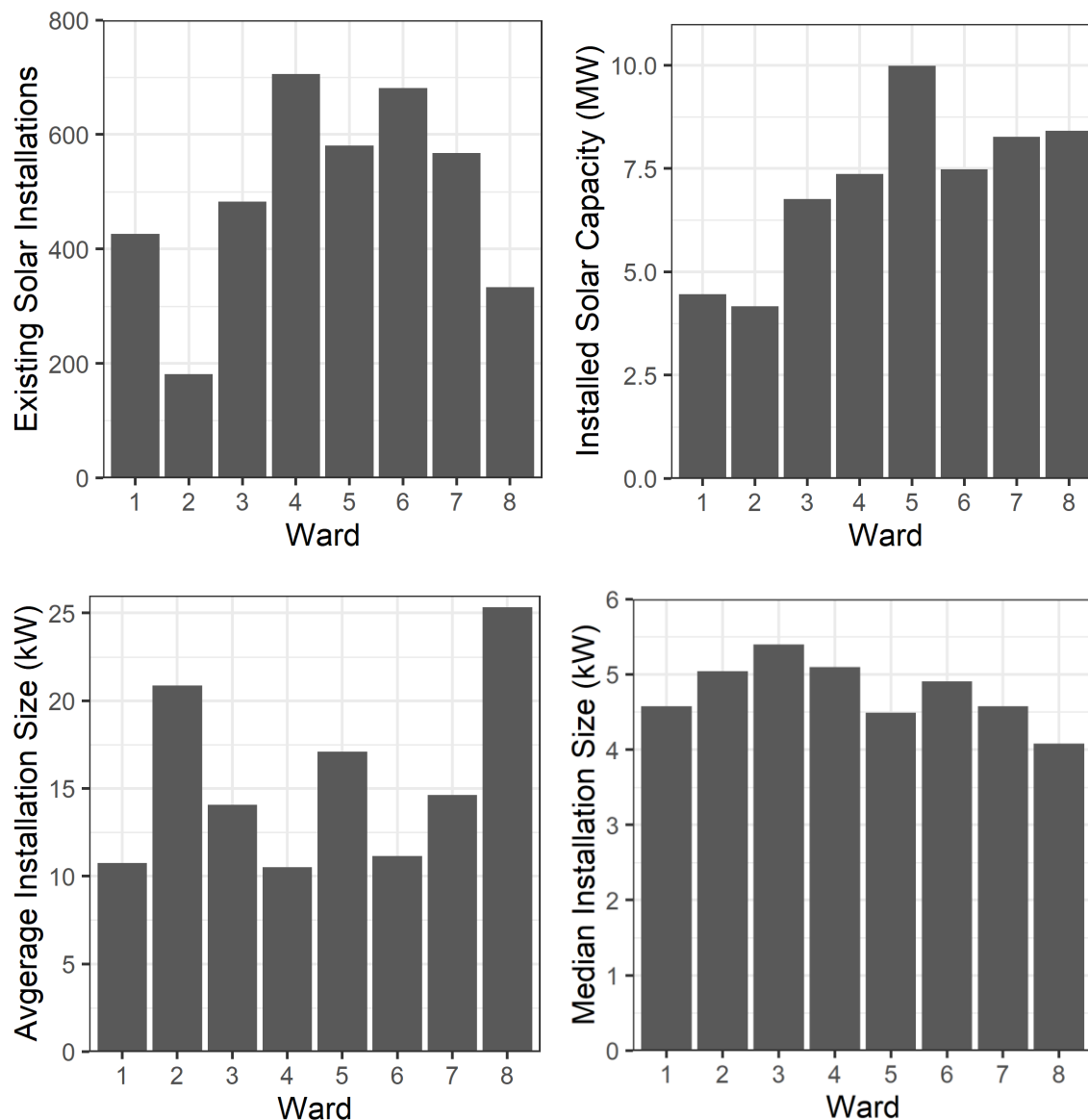
Figure 6. Existing number of solar installations (top left), installed capacity (top right), average solar installation size (bottom left), and median installation size (bottom right) by ward through end of 2018
