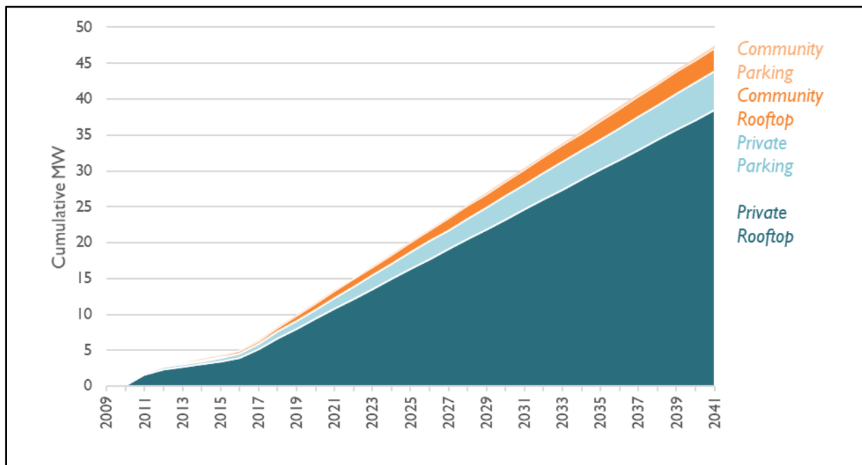
Figure 24. Ward 2 Low projection solar potential by installation type
